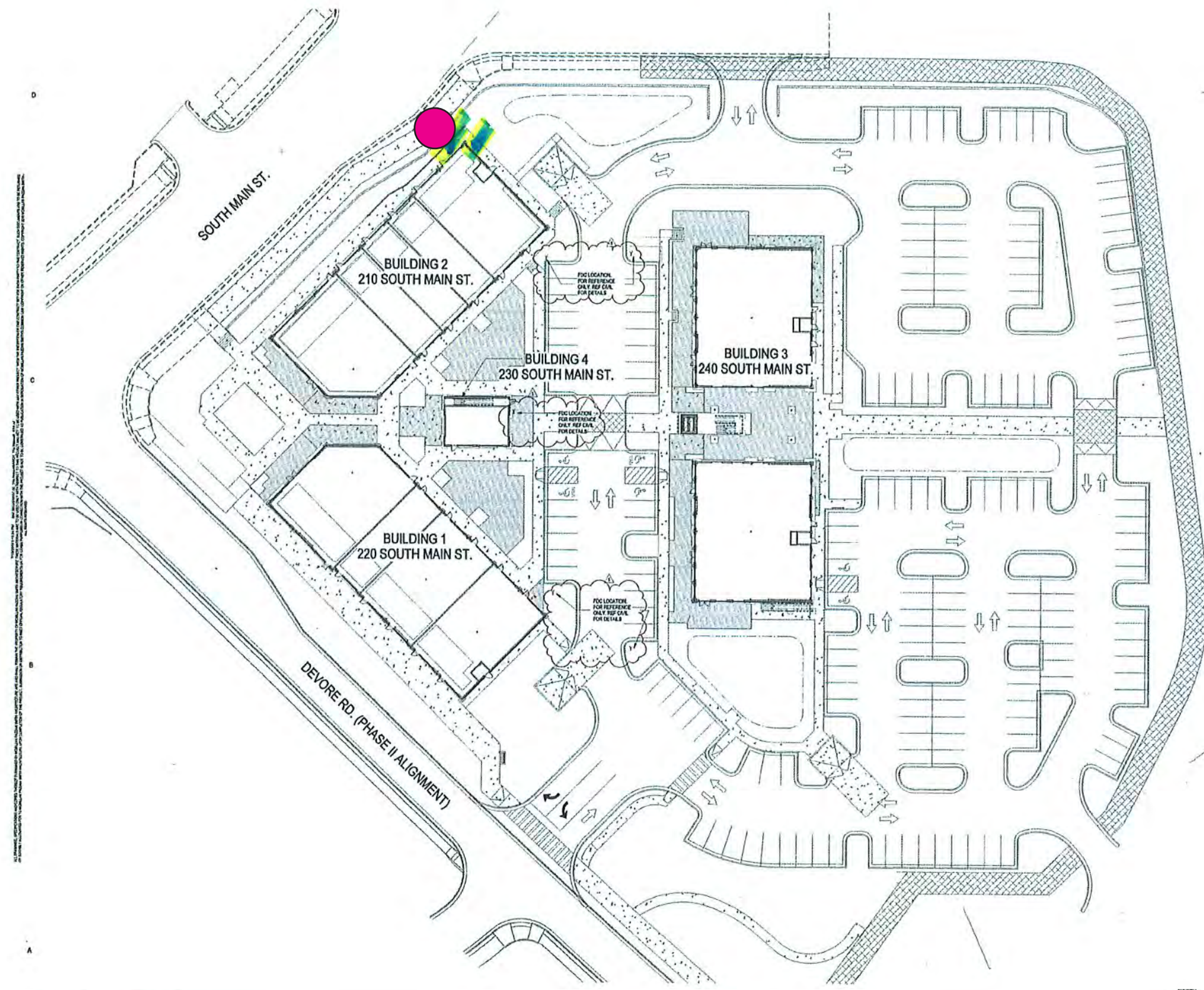
1 ARCHITECTURAL SITE PLAN A010 3/6/19
