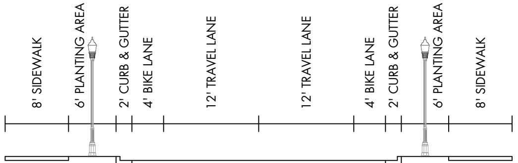
TYPICAL SECTION
