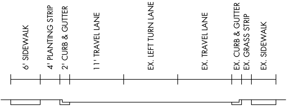
TYPICAL SECTION (LOOKING TOWARDS WESTSIDE PARKWAY)
