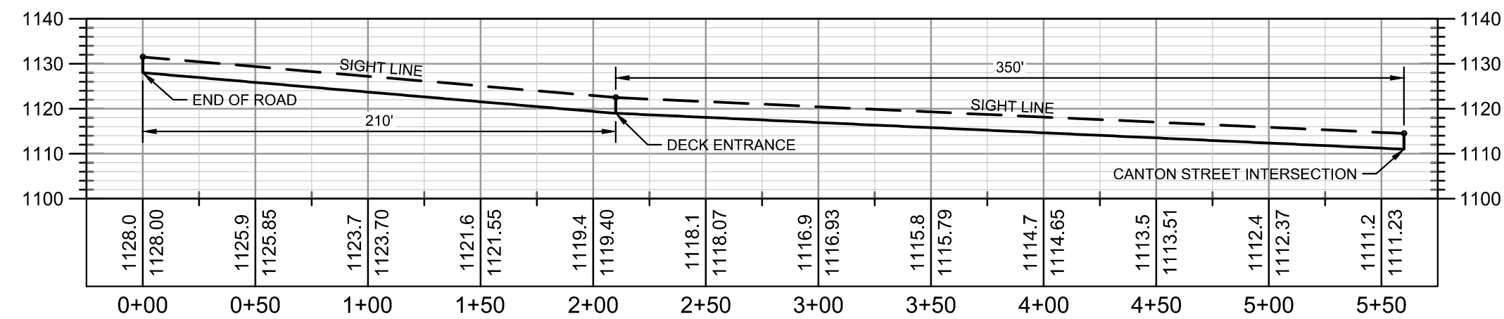
PROFILE VIEW DECK ENTRANCE SIGHT DISTANCE PROFILE 1" = 30' HORIZ. 1" = 15' VERT.
